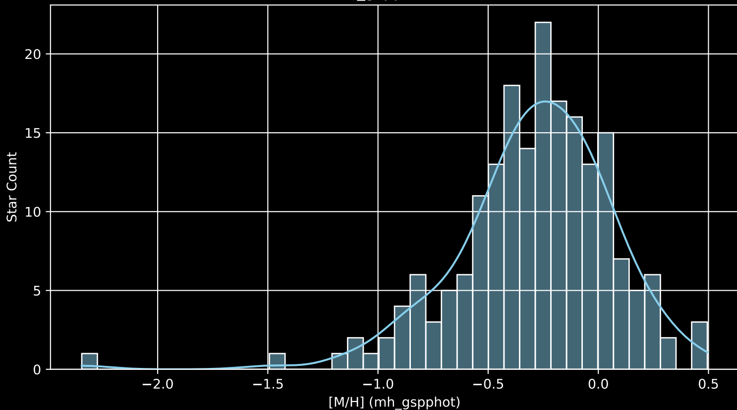
APOGEE DR17 Field: [K2_C4_173-32_btx [M/H] (mh_gspphot) (n= 194)
