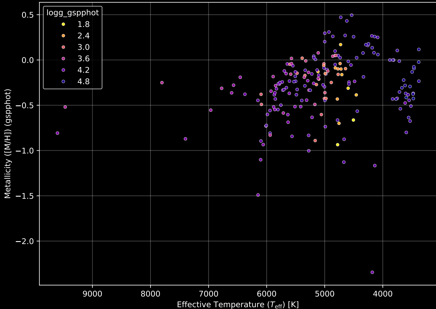
APOGEE DR17 Field: [K2_C4_173-32_btx] Stellar Population Parameters (n= 194)
