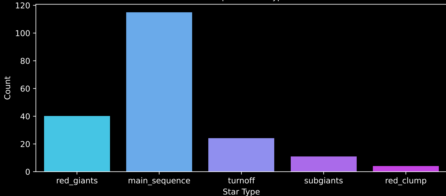
APOGEE DR17 Field: [K2_C4_173-32_btx] Count plot of Star Type
