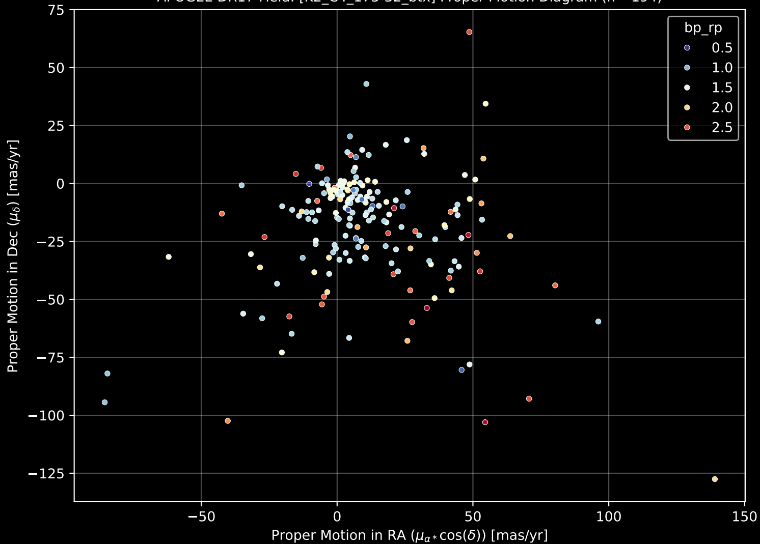
APOGEE DR17 Field: [K2_C4_173-32_btx] Proper Motion Diagram (n= 194)
