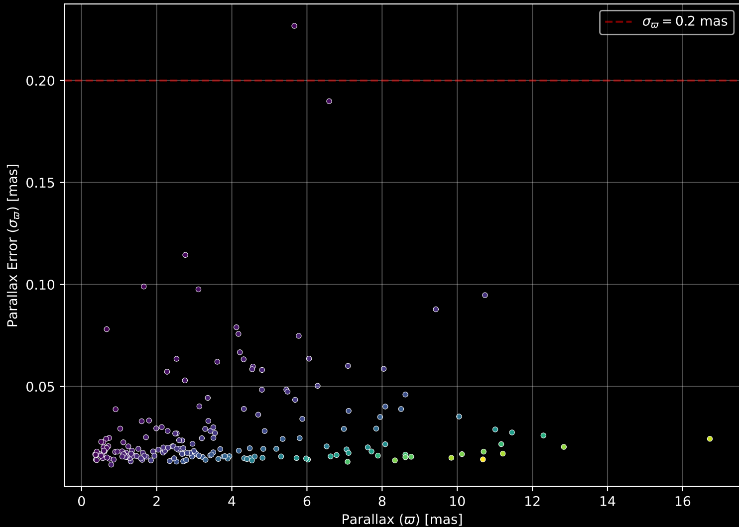
APOGEE DR17 Field: [K2_C4_173-32_btx] Parallax Quality (n= 194)
