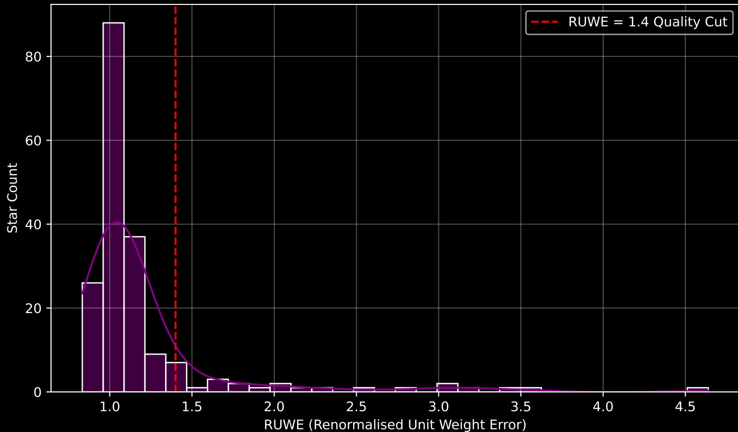
GAPOGEE DR17 Field [K2_C4_173-32_btx] RUWE Distribution (n= 186)
