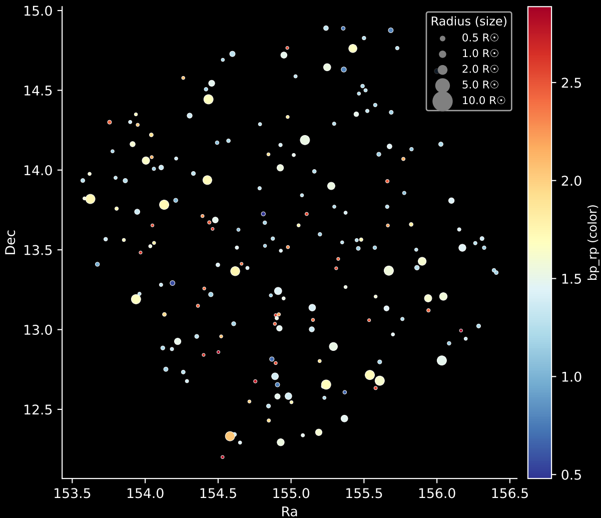
APOGEE DR17 Field: [K2_C4_173-32_btx] Stars: 194
